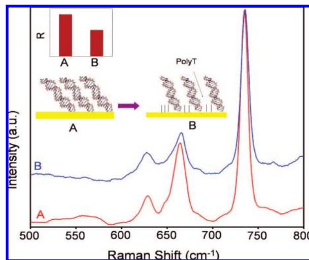
Figure 3. DNA tilt due to incubation with polyT: (a) SERS spectra of SA 20 N1(2.5 μM) before polyT incubation, (b) SERS spectra of SA 20 N1 after polyT incubation, (c) bar plot showing the adenine/guanine peak intensity ratio before and after polyT incubation. Insets are schematics depicting the DNA orientation variation caused by polyT incubation.
